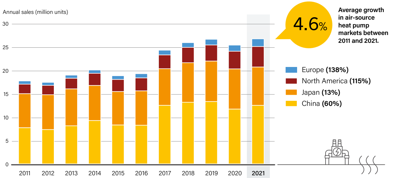
FIGURE 31. Air-Source Heat Pump Annual Sales, Selected Markets, 2011-2021
